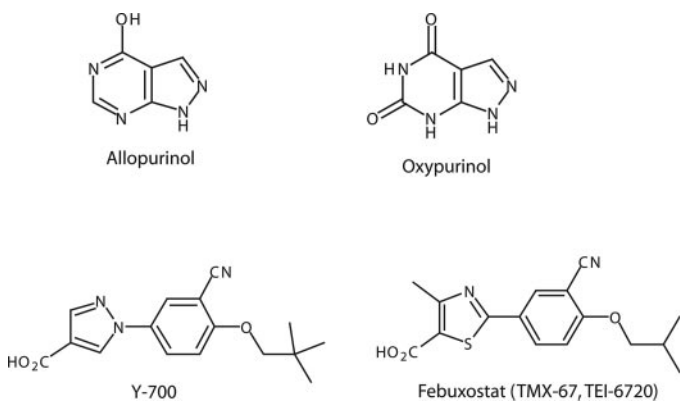
FIG. 3. Chemical structures of selected xanthine oxidase inhibitors.
