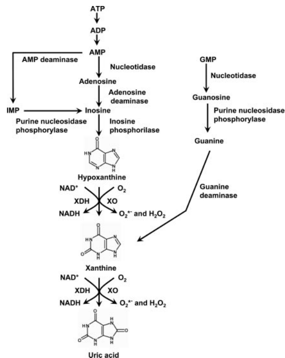
FIG. 1. Schematic diagram of the purine degradation pathway.
